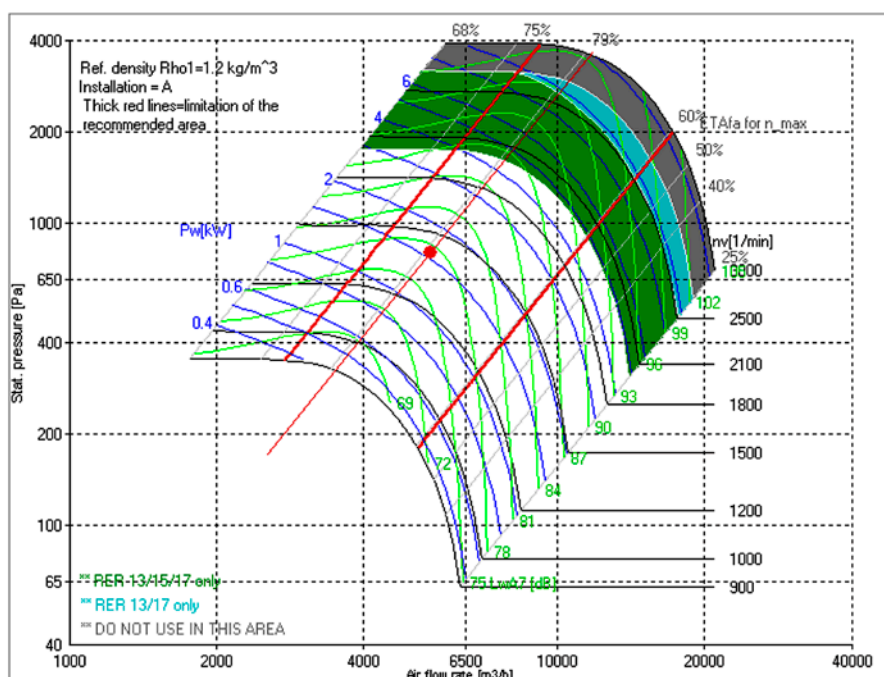
Regeneration Fan Curve for the 30000 VRF
